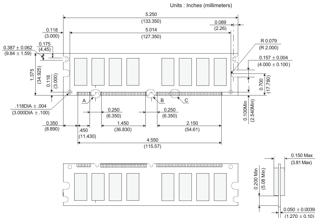
Figure 1: KVR100X64C3/512 168-Pin SDRAM Module
